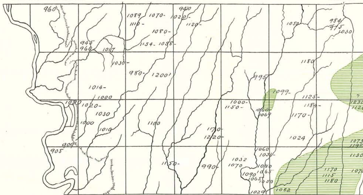
GEOLOGICAL MAP OF POTTAWATTAMIE COUNTY.
