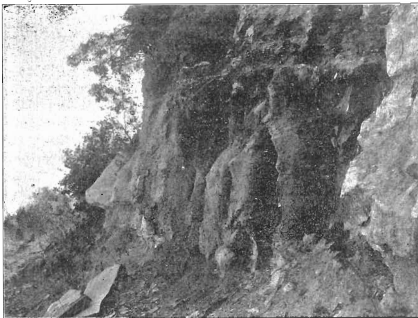
FIG. 68. Contact between the Saint Louis limestone, 1, and Coal Measures, 2. Three miles above Ottumwa.
