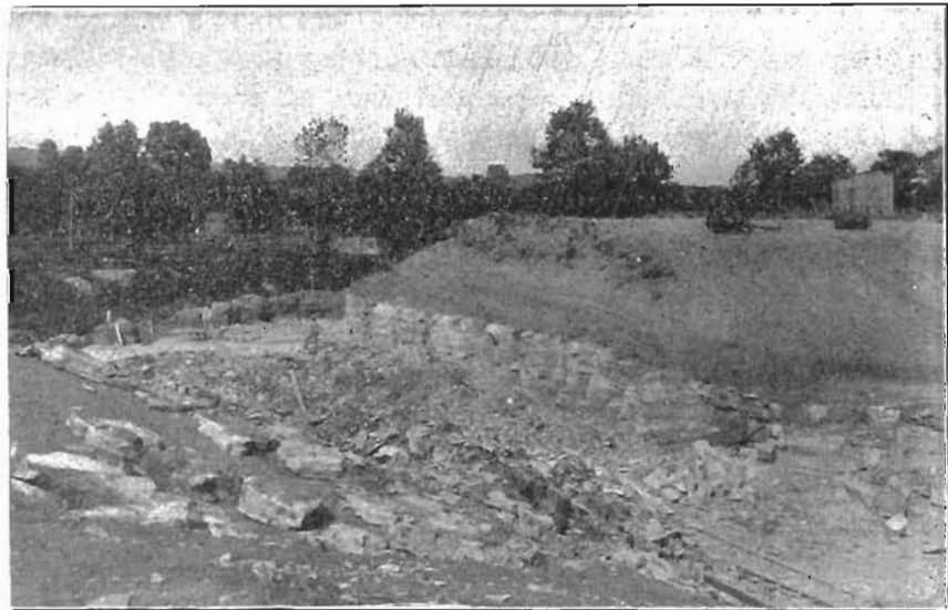
FIG. 75. Quarry of Andrew Lames at Dudley, showing the Saint Louis beds overlain by drift.
