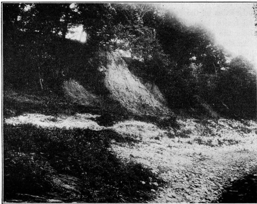
Figure 27. Exposure of Verdi beds, Saint Louis limestone, in left bank of the Skunk river, northwest quarter of section 36, Sugar Creek township.
